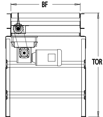
Underhung Drive with Leg Supports
